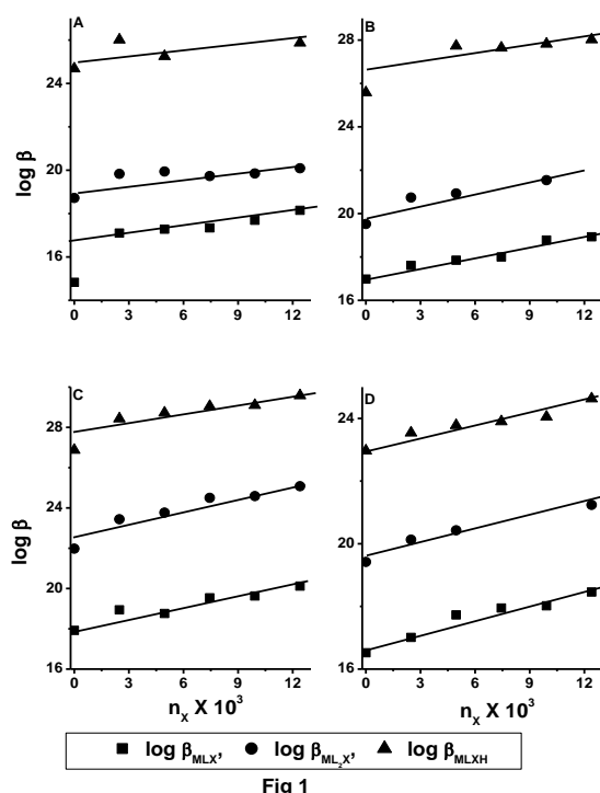
Fig. 1 Variation of stability constant of ternary complexes with mole fraction of CTAB (A) Co(II) B) Ni(II) C) Cu(II) and D) Zn(II).
