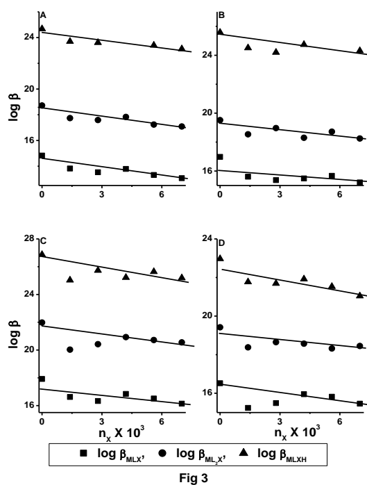
Fig. 3 Variation of stability constant of ternary complexes with mole fraction of TX100 (A) Co(II) B) Ni(II) C) Cu(II) and D) Zn(II)
