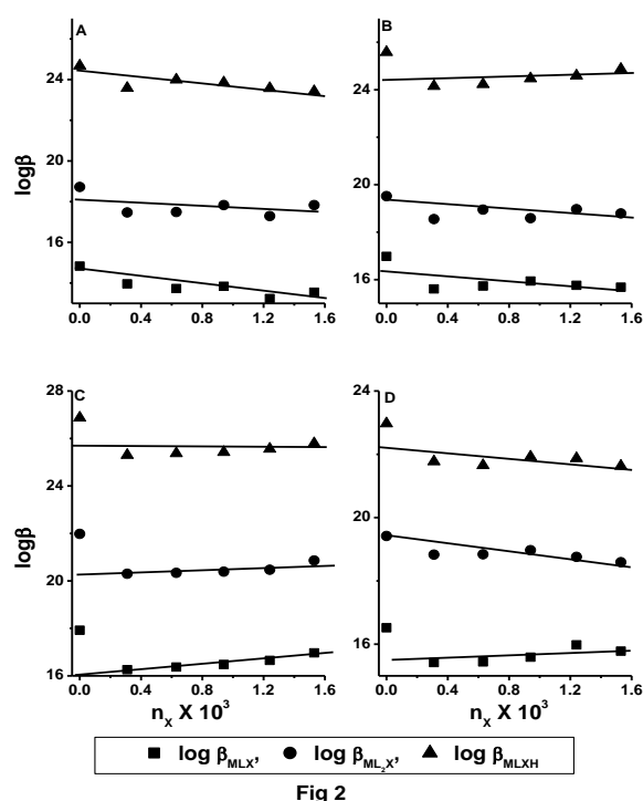
Fig. 2 Variation of stability constant of ternary complexes with mole fraction of SLS (A) Co(II) B) Ni(II) C) Cu(II) and D) Zn(II).
