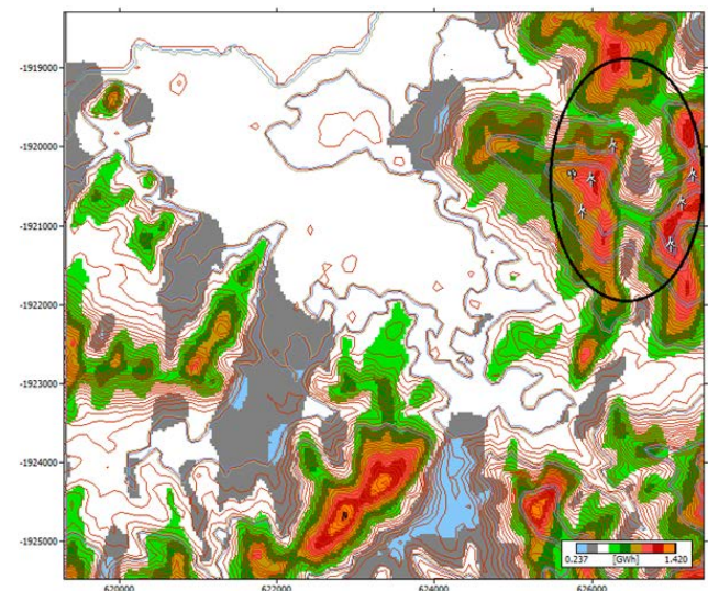
Figure 13 Wind farm layout at Tuvavatu
