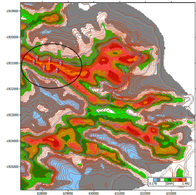
Figure 12 Wind farm layout at Navolau
