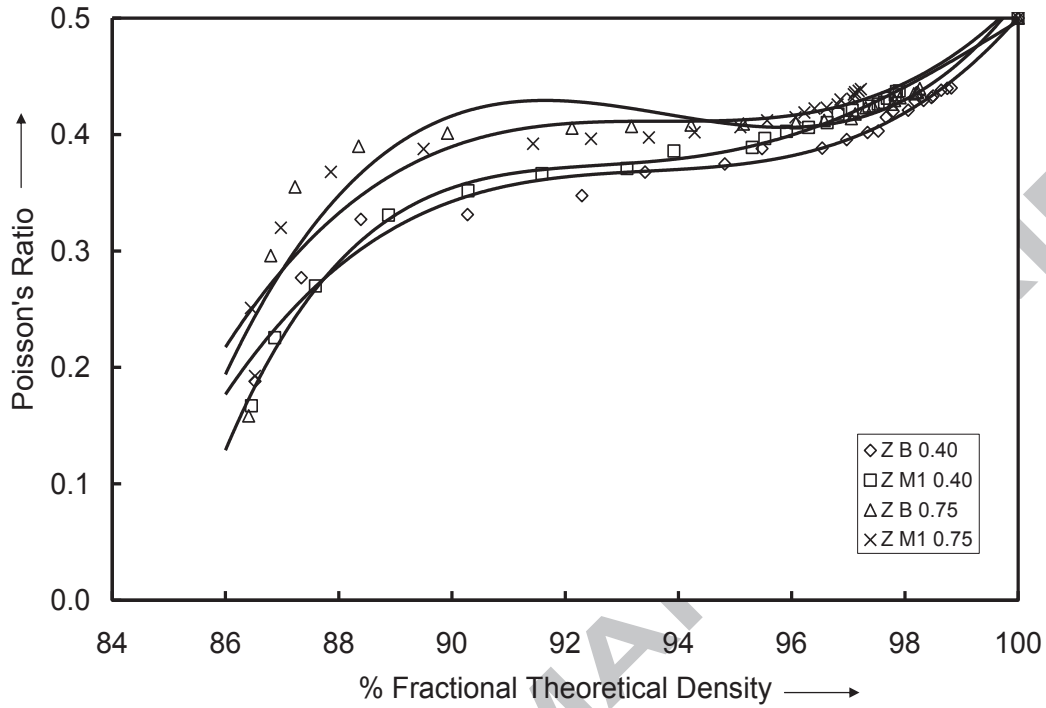
Figure 5: The relationship between Poisson's ratio and percentage fractional theoretical density
