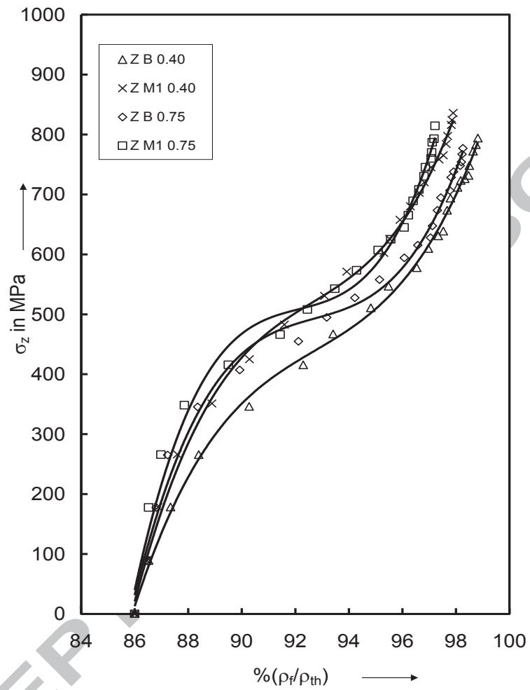
Figure 7: The relationship between \sigma_z and \%(\rho_f/\rho_{th})
