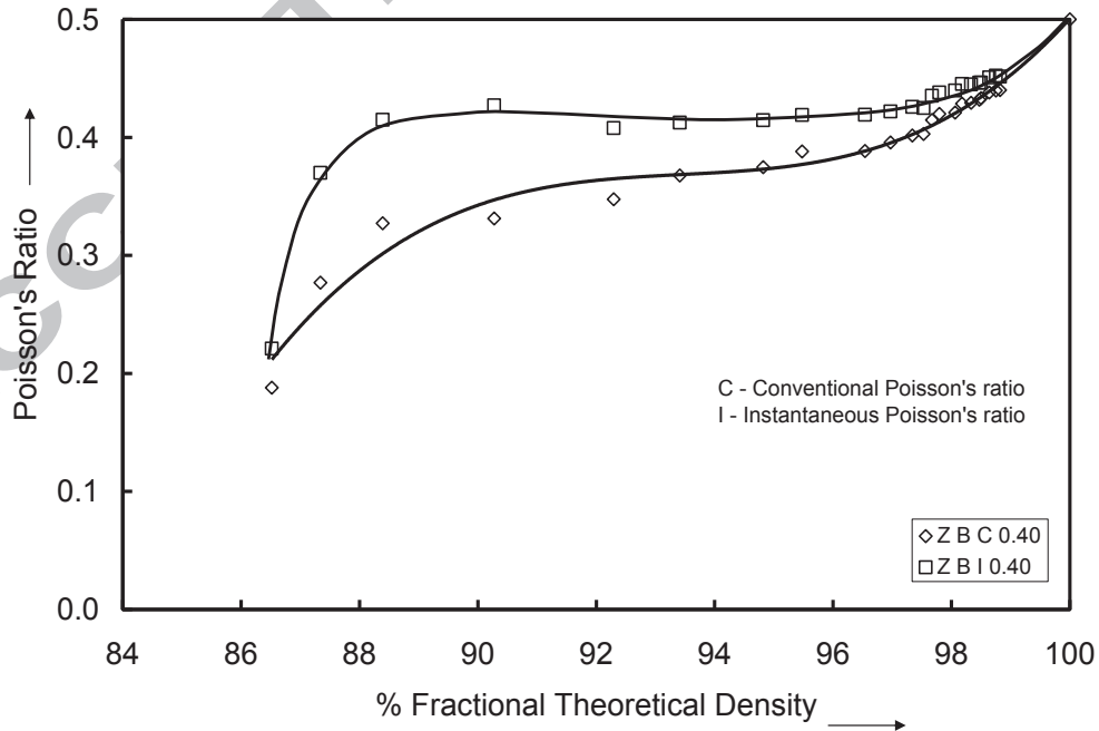
Figure 6(a): Variation of Poisson's ratio and percentage fractional theoretical density for Fe-0.8%C steel preforms of 0.40 aspect ratio
