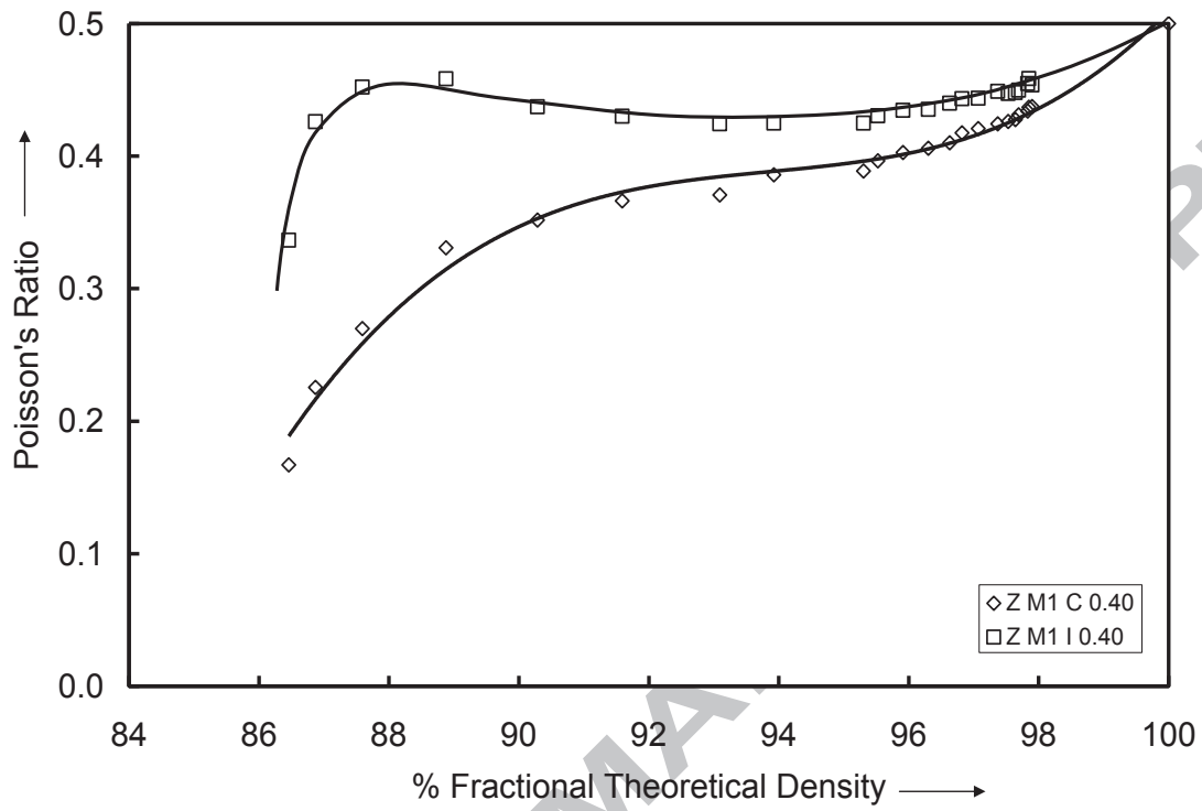
Figure 6(b): Variation of Poisson's ratio and percentage fractional theoretical density for Fe-0.8%C-1.0%Mo steel preforms of 0.40 aspect ratio
