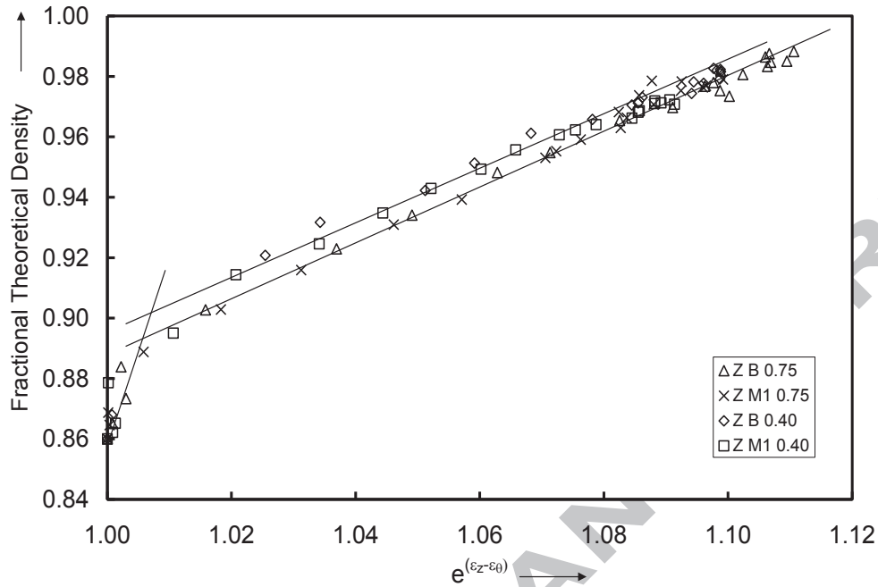
Figure 3: The relationship between fractional theoretical density and e^{\epsilon_z - \epsilon_\theta}
