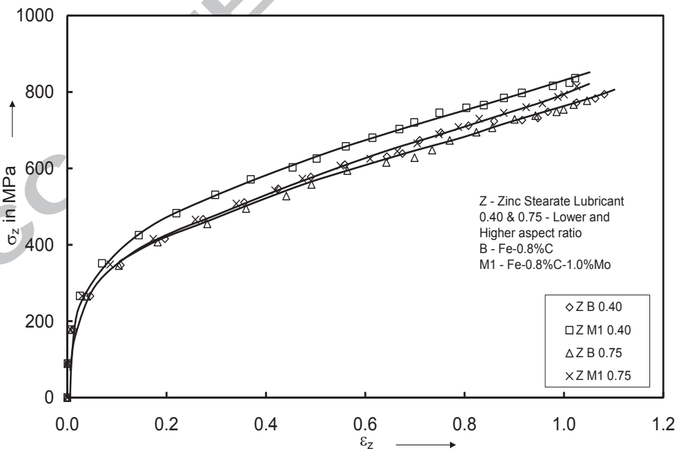
Figure 2: The relationship between \sigma_z and \epsilon_z
