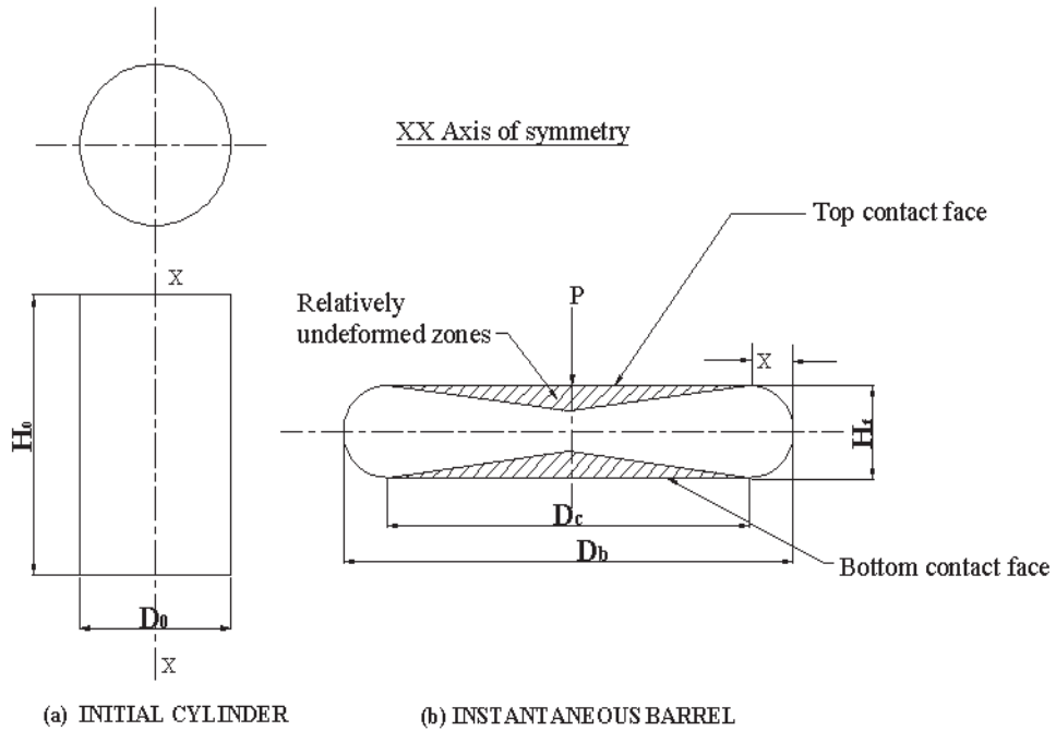
Figure 1: Schematic representation of upset forging test specimen before and after deformation
