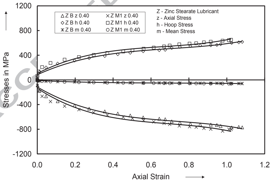
Figure 4: The relationship between various stresses and axial strain for a given aspect ratio of 0.40
