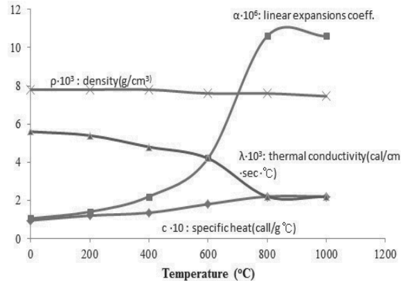
Fig. 3. Thermo-physical properties of SS400 steel as a function of temperature
