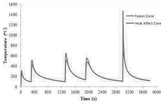
Fig. 8. FEM FZ and HAZ Temperature histories of each pass for multi-pass welding
