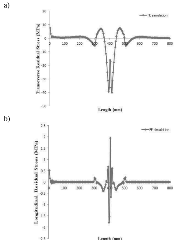
Fig. 10. Transverse and Longitudinal residual stress at the bottom surface of the weld plate, a) Transverse residual stress, b) Longitudinal residual stress
