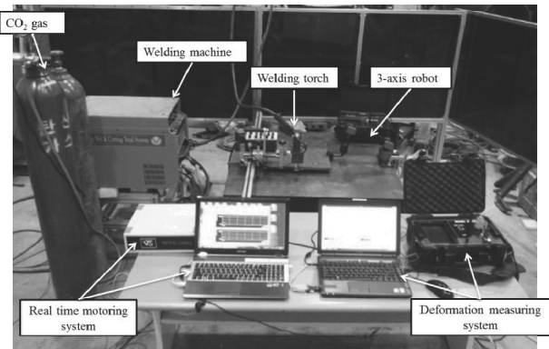
Fig. 6. Multi-pass GMA welding experiment setup
