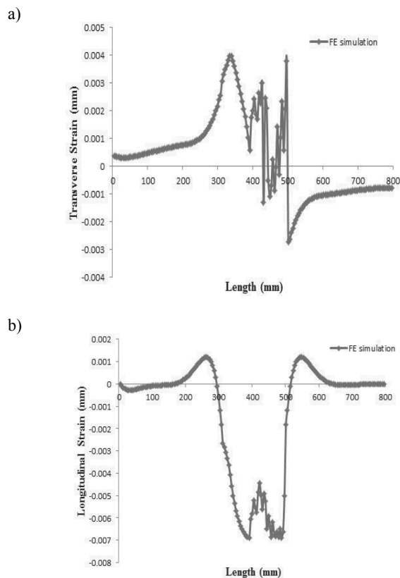
Fig. 11. Transverse and longitudinal strain distribution on the welded plate, a) Transverse stress, b) Longitudinal stress
