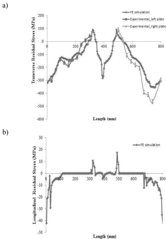
Fig. 9. Transverse and Longitudinal residual stress at the top surface of the weld plate, a) Transverse residual stress. b) Longitudinal residual stress
