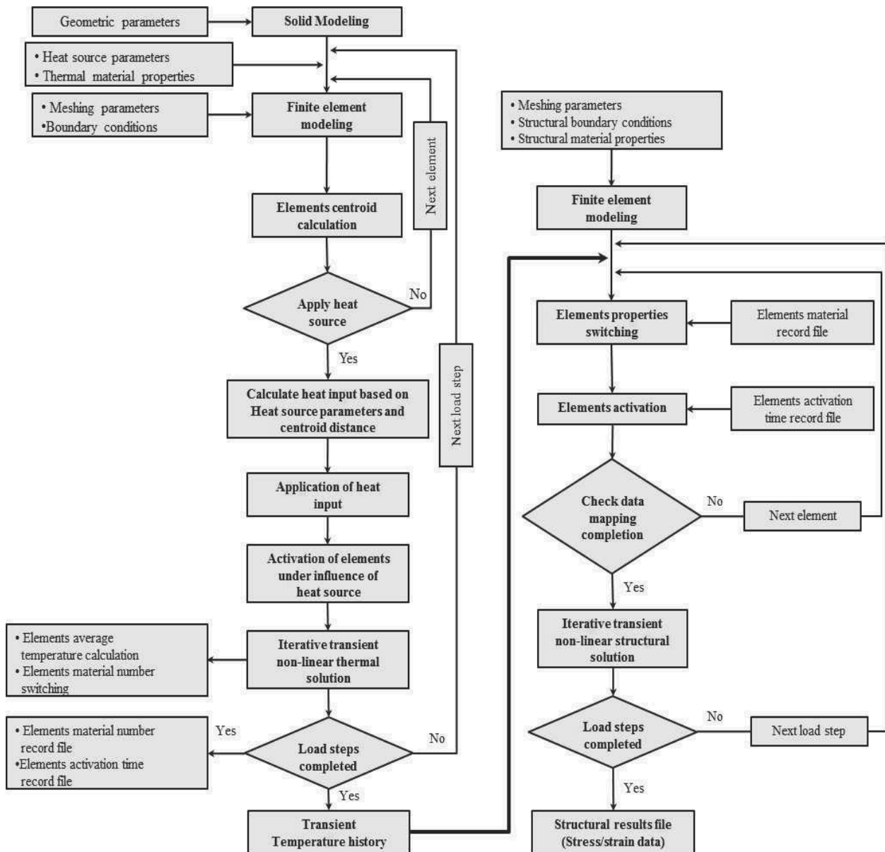
Fig. 1. Flow chart for FEM coupled thermo-mechanical phenomenon
