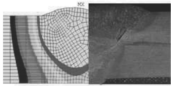
Fig. 7. Comparison of FE simulation and experimental bead geometry
