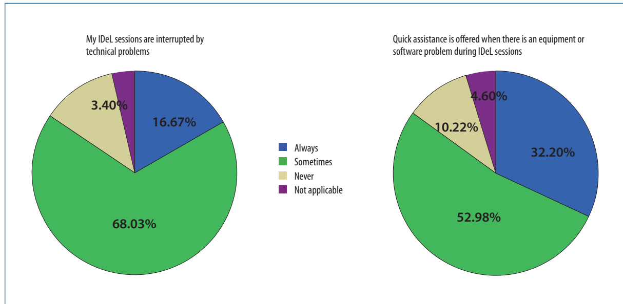
Figure 2C: ICT issues
