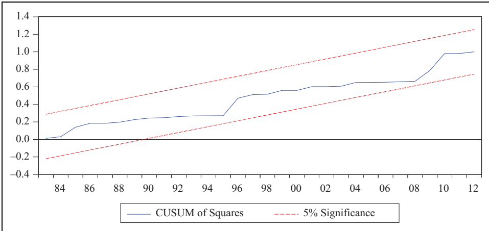
Figure 2. Plot of CUSUMQ of recursive residuals. The straight lines represent critical bounds at 5% significance level. CUSUMQ: cumulative sum of squares.
