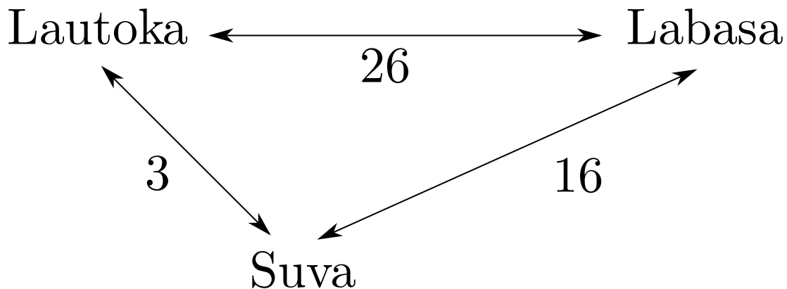
Figure 1.1: The travelling salesperson problem
