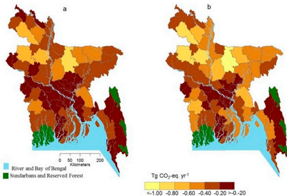
Figure 4. Map of Bangladesh showing (a) annual soil organic carbon (SOC) stock changes (Tg carbon dioxide \text{CO}_2 -eq. \text{year}^{-1} ) and (b) average net greenhouse gas (GHG) balances (Tg \text{CO}_2 -eq. \text{year}^{-1} ) from total rice harvested area under integrated management practices (IM) for the period 1996–2015. Unit and legend for Figure 4b is similar to Figure 4a.
