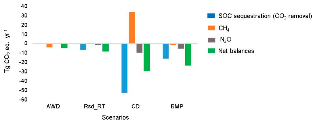
Figure 5. Annual balances (Tg carbon dioxide, \text{CO}_2 -eq. \text{year}^{-1} ) considering soil organic carbon (SOC) stock changes (represented as a \text{CO}_2 removal), methane and nitrous oxide emissions under the four selected mitigation scenarios in the harvested rice area of Bangladesh. Negative values indicate an increase in SOC sequestration or a decrease in net greenhouse gas (GHG) emissions; positive values indicate a decrease in SOC sequestration or an increase in net GHG emissions. AWD: Alternate wet and drying, Rsd_RT: 15% residue removal with reduced tillage, CD: Cow dung, IM: Integrated management practices.
