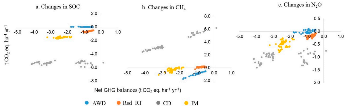
Figure 1. Simulated net greenhouse gas (GHG) balances ( \text{t CO}_2\text{-eq. ha}^{-1} \text{ year}^{-1} ) related to changes from the baseline management in (a) soil organic carbon (SOC) stock (carbon dioxide, CO 2 removal), (b) methane (CH 4 ) and (c) nitrous oxide (N 2 O) emissions (all are in \text{t CO}_2\text{-eq. ha}^{-1} \text{ year}^{-1} ) for 64 districts in Bangladesh. Each point represents the change in one district ( n = 64 ). AWD: Alternate wet and drying, Rsd_RT: 15% residue removal with reduced tillage, CD: Cow dung, IM: Integrated management practices. Note that the scale of both x and y axes differ.
