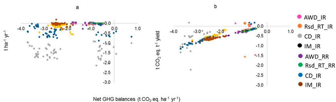
Figure 2. Simulated net greenhouse gas (GHG) balances with (a) yield in two crop growing seasons and (b) GHG emission intensity under different management activity in Bangladeshi double rice cropland soil. Each point represents the change in one district ( n = 64 ). Y_IR: Yield for irrigated rice, Y_RR_Yield for rainfed rice. AWD: Alternate wet and drying, Rsd_RT: 15% residue removal with reduced tillage, CD: cow dung, IM: Integrated management practices.
