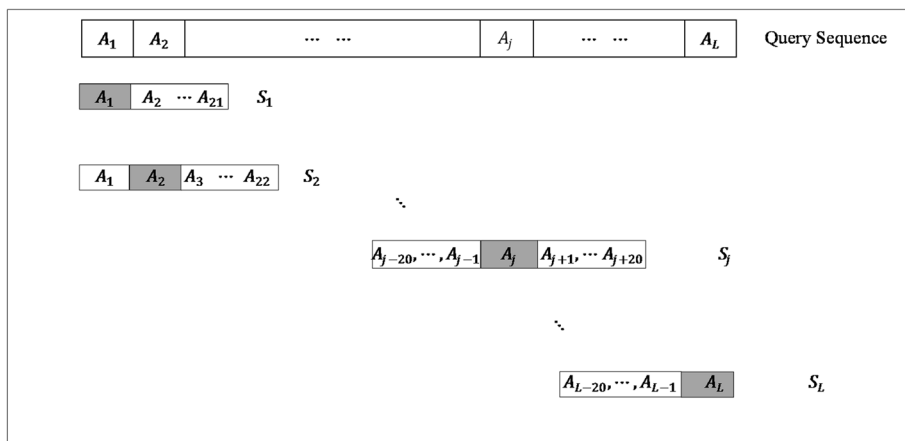
Fig. 2 Schematic illustration of extracting samples to score a query sequence. A_j is the j -th amino acid in the query sequence and L refers to the length of the query protein sequence
