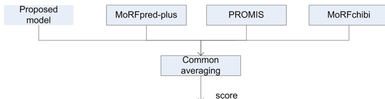
Fig. 3 Combined model. MoRFpred-plus and PROMIS are our predictors while we download MoRFchibi predictor and integrate it with our proposed model
