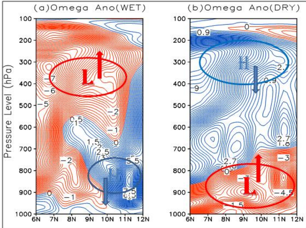
Fig. 16: The mean May-October omega ( \omega ) anomaly ( 10^{-3}\text{Pas}^{-1} ) over Togo at longitude 1^\circ\text{E} during (a) wet years (1989, 1991, 1995, 2007) and (b) dry years (1982, 1983, 1992, 2001, 2006). Arrows indicate high (blue, H)/Low (red, L) pressure centers and Sinking/Rising air motion.
