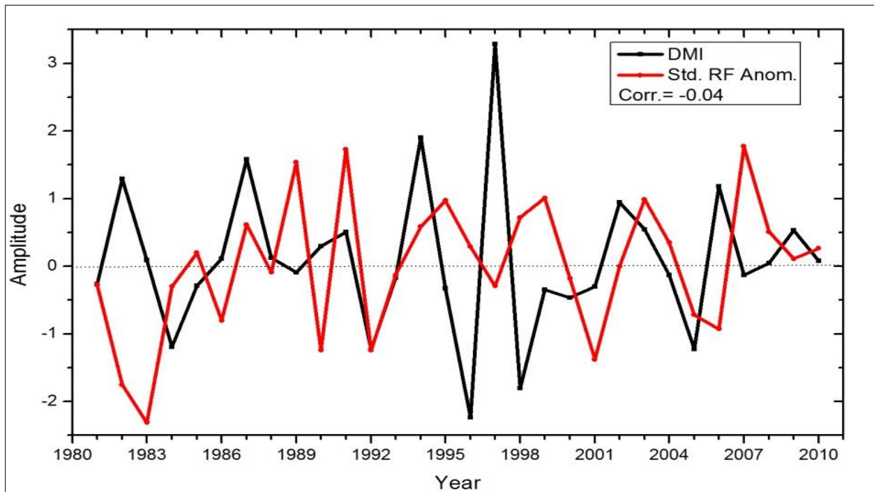
Fig. 14: Inter-annual variability of standardized May-October RF anomaly over Togo and IOD index during the period 1981-2010 (correlation between DMI and RF is -0.04).
