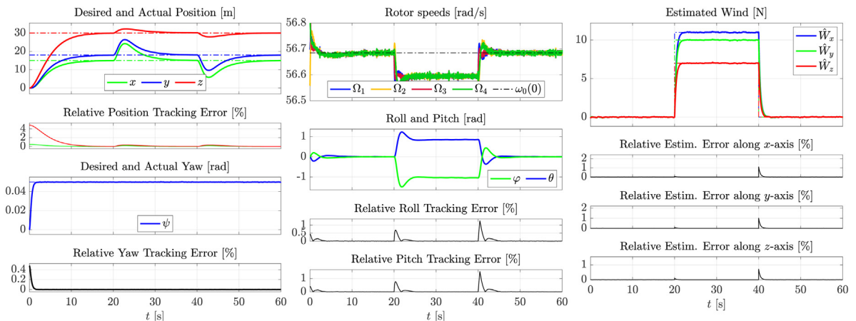
Fig. 7. ROS/Gazebo-based testing of the controlled Erlecopter, closed in the loop with the proposed UIO and linear controller, under the occurrence of a sudden and large step-wise wind. A step-wise wind force signal of storm category with magnitude N = (11, 10, 7)^T N is successfully reconstructed and its effect compensated. Controller gains are \lambda_a = 0.4 and \lambda_p = 4 . Steady-state roll and pitch angles are about 0.86 rad (49.27 degrees) and -0.94 rad ( -53.85 degrees), respectively, which are clearly far from the small angle hypothesis. This reveals a large applicability of the proposed method.
