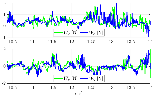
Fig. 10. Experimental results during a hovering task. The UIO filter shows a sufficient level of accuracy in the wind estimation.
