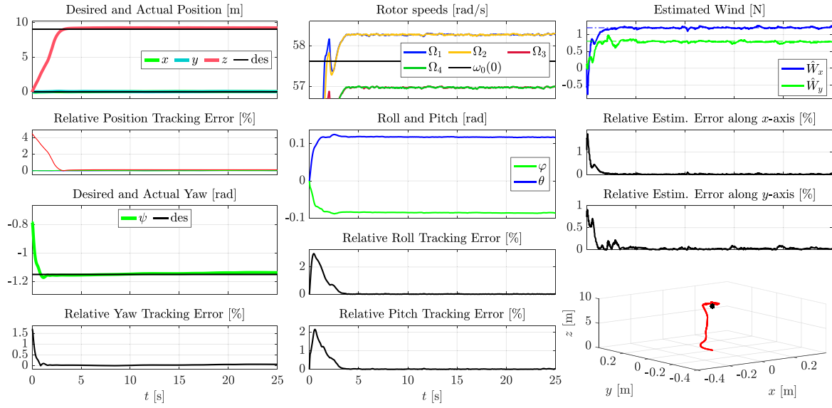
Fig. 4. ROS/Gazebo-based validation of the hybrid solution with the proposed UIO filter, designed for a horizontal wind scenario, used in combination with the Ardupilot controller. The Erlecopter is required to takeoff up to x_d = 0 m, y_d = 0 m, z_d = 9 m, with required yaw of \psi_d = -1.15 rad, while the wind amplitude is N = (\bar{W}_x, \bar{W}_y) = (1.2, 0.8) N.
