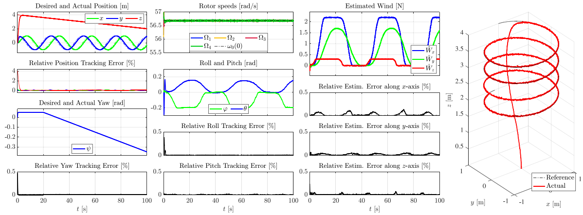
Fig. 5. ROS/Gazebo SITL validation with a general wind gust of force components N = (\bar{W}_x, \bar{W}_y, \bar{W}_z) = (2.20, 1.70, 0.35) N. The UIO filter can estimate the wind with a high accuracy and the linear controller allows accurate tracking of a spiral trajectory.
