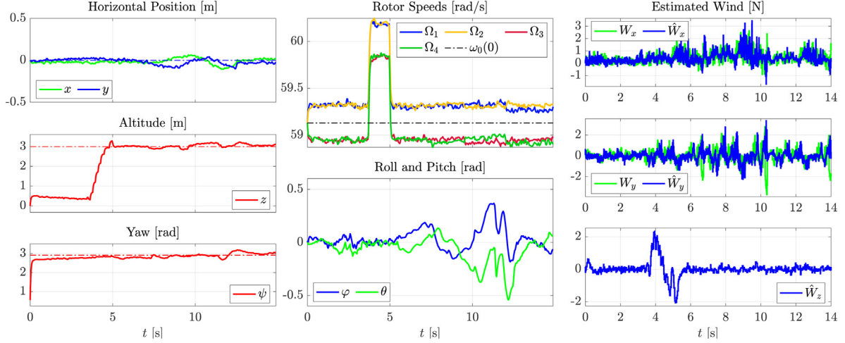
Fig. 9. Experimental results during a point-to-point motion task where the aircraft autonomously hovers at 0.5 m, then quickly reaches 3 meters, and finally continues to hover. Apart from the very fast translation phase (for t \in [3.6, 5.1] s), during which the quasi-hovering assumption is temporarily violated and the UIO filter detects a virtual upward vertical force, the filter itself correctly estimates the wind components as expected and the proposed controller maintains the desired position.
