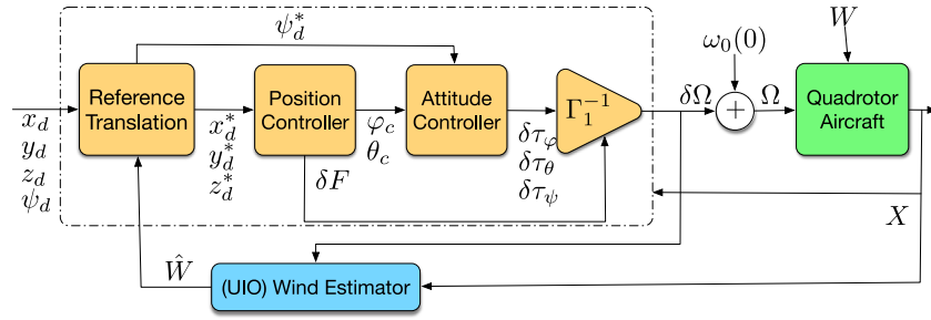
Fig. 2. Architecture of the proposed controller with cascaded position and attitude regulation and wind estimation and compensation. The measured state X and rotor speed variations \delta\Omega are used to obtain wind estimates \hat{W} , which are mapped to the proper translated references, x_d^* , y_d^* , z_d^* , and \psi_d^* , through Eq. (33) and (36); these position references are then used to derive commanded roll \varphi_c and pitch \theta_c , which, along with the yaw reference are converted to the required thrust variation \delta F and torque variations, \delta\tau_\varphi , \delta\tau_\theta , \delta\tau_\psi ; finally these quantities are converted to rotor speed variations and, by adding \omega_0(0) , to the required absolute rotor speeds \Omega .
