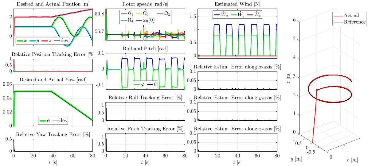
Fig. 3. Results from a Matlab/Simulink simulation run with horizontal wind gusts. The controlled quadrotor quickly reaches a desired position of x_d = 1 m, y_d = 1 m, z_d = 2 m and \psi_d = 5 \cdot 10^{-2} rad. As the wind-gust series starts at t = 15 s, the UIO rapidly reconstructs the wind-force component signals and provides their values to the pose recovery controller. The controller commands rotor speed signals that ensure a sufficient total thrust and lead to suitable roll and pitch angles. From t = 38 s, the quadrotor starts tracking a spiral trajectory, while the wind-gust series continues to be present. It can be observed that the small-value hypothesis for the roll and pitch angles is always satisfied. Gust amplitudes are W_{x,m} = 1.2 N and W_{y,m} = 0.8 N, gust lengths are d_{x,m} = d_{y,m} = 0.5 m, and gust frequencies are f_x = f_y = 0.5 rad/s. State and unknown wind estimates are very accurate.
