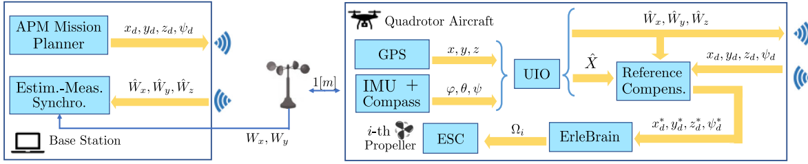
Fig. 8. Data-flow in the experimental setup on the aircraft system and the base station. ROS nodes and topics are represented by blocks and arrows, respectively. Ground-truth information about the norm and direction of the horizontal wind-speed is measured by a 3-cup rotor sensor and a wind vane, placed at around 1-meter distance and the same height of the desired hovering position.
