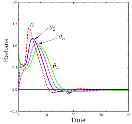
Fig. 5 Orientations of the tractor and its trailers
