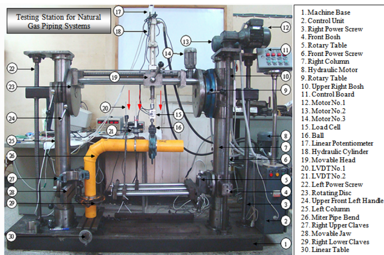
Fig. 1. Photo of Testing Machine for Natural Gas Piping Systems (NGPS)
