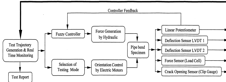
Fig. 3. Block Diagram for Control Loop and Signal Monitoring Loop
