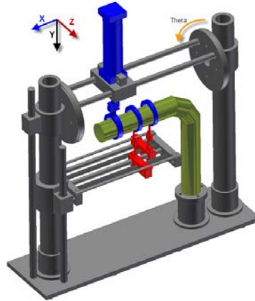
Fig. 2. Three Dimensions Model for Special Testing Machine (STM)
