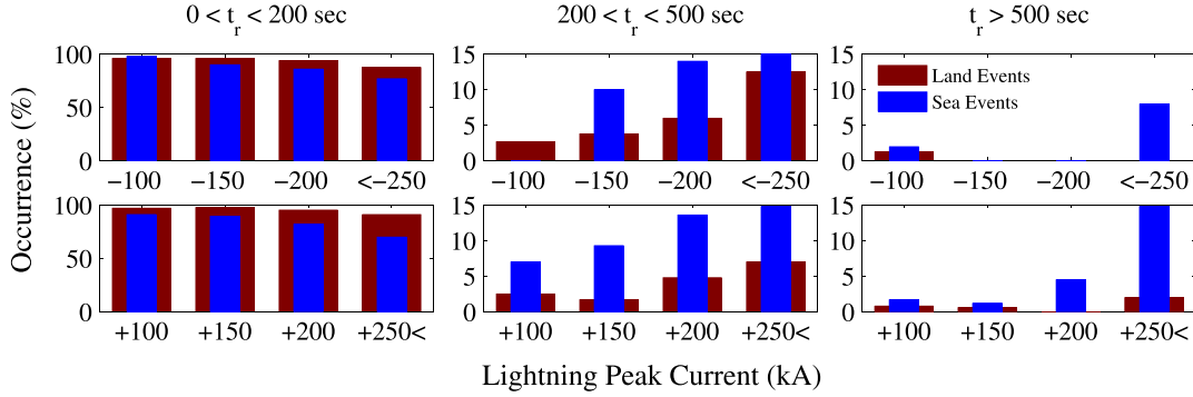
Figure 8. Distribution of peak current of the causative lightning discharges as a function of the recovery duration ( t_r ) of Early VLF events. The figure shows that as the peak current of lightning increases, the occurrence rate of Early VLF events with long-enduring recovery increases.
