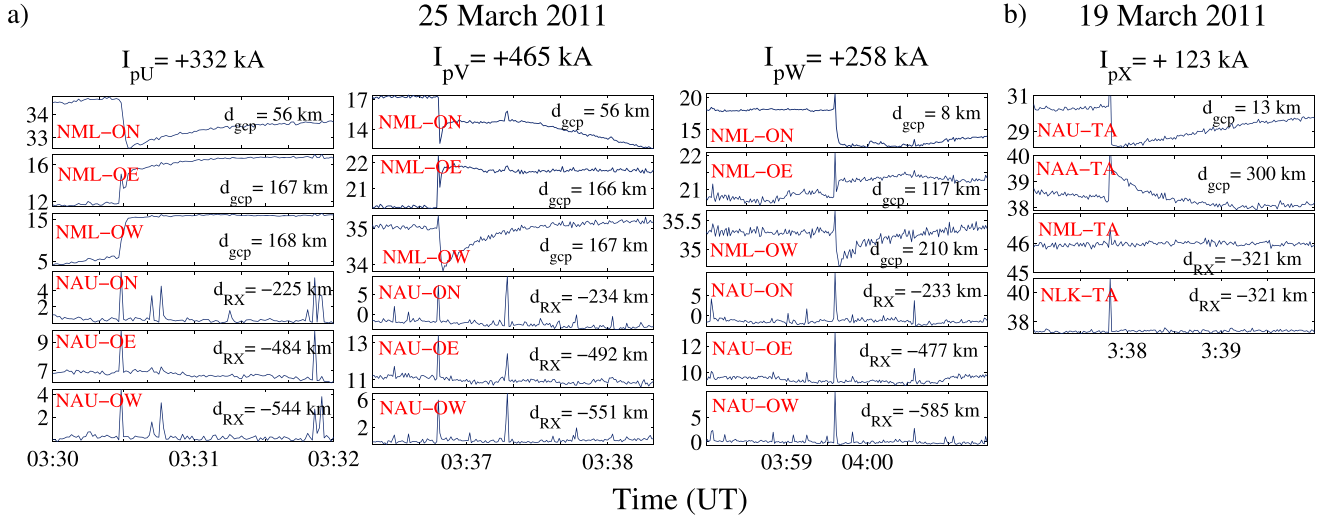
Figure 6. (a) Multiple VLF signatures of amplitude perturbations observed on 25 March 2011 in association with three very large peak current +CG lightning discharges ranged from +258 to +465 kA. A one-to-one correlation between these very large peak current +CG discharges and VLF forward scatter events was found. (b) A +123 kA peak current on 19 March 2011 occurred near ( d_{RX} = 321 km) Taylor VLF receiver. This large peak current lightning perturbed the NAA and NAU VLF signals, indicating forward scattering Early VLF signal perturbations, but it could not perturb the NML and NLK signals located in backward directions.
