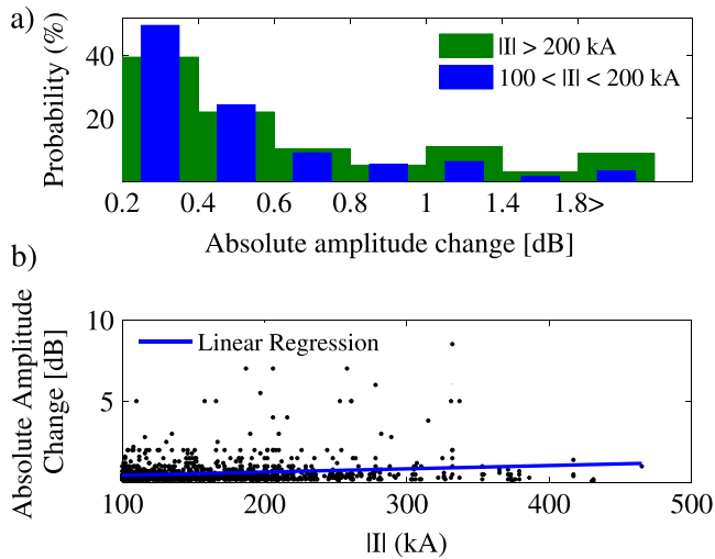
Figure 9. (a) Distribution of amplitude change in decibel associated with Early VLF events. (b) The scatterplot of amplitude perturbations associated with all detected Early VLF events, together with a linear regression and correlation coefficient analysis.
