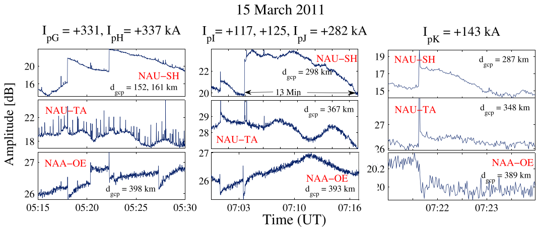
Figure 4. Early VLF events observed on 15 March 2011 between 0500 and 0730 UT. The lightning discharges responsible for these events had peak current magnitude above +100 kA. These high peak current discharges generated five large amplitude perturbations on the NAU-SH path with amplitude perturbations ranging from \sim 0.8 to 5 dB and several smaller sharp amplitude changes on the NAU-TA and NAA-OE signal paths \sim 0.2 – 0.4 dB in amplitude. It is evident from the figure that Early VLF events caused by high peak current lightning discharges can be observed when the disturbance region is \sim 400 km from the GCP.
