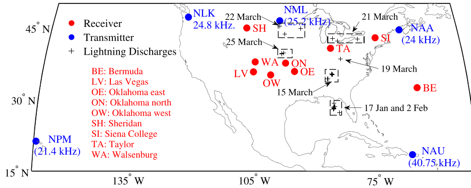
Figure 1. Geographic locations of five U.S. naval VLF transmitters, together with the causative lightning discharges occurred on 17 January, 2 February, and 15, 19, 21, 22, and 25 March 2011.
