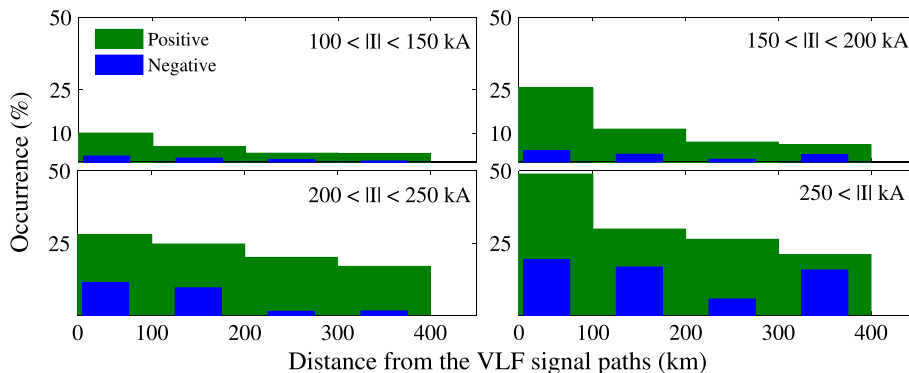
Figure 7. Probability of generating an Early VLF events as a function of the peak current magnitude of the causative lightning discharges and distance of stroke location from the VLF signal paths, for data between 1 January to 2 February 2011 and from 1 to 25 March 2011. It is evident from the figure that the apparent size of the ionospheric disturbance grows larger for larger peak currents.
