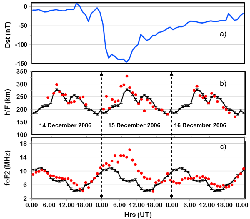
Figure 6. (a) Variation in Dst index for the geomagnetic storm of 14–16 December 2006. (b, c) Corresponding hourly variation of h' F and f o F 2 (red solid points) over Niue (19.06.2°S, 169.93°W). The monthly median values of these parameters with standard errors are shown by solid lines.
