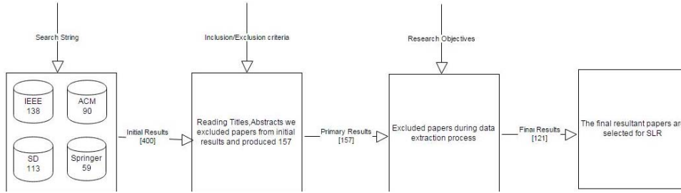
Figure 1 Selection process
